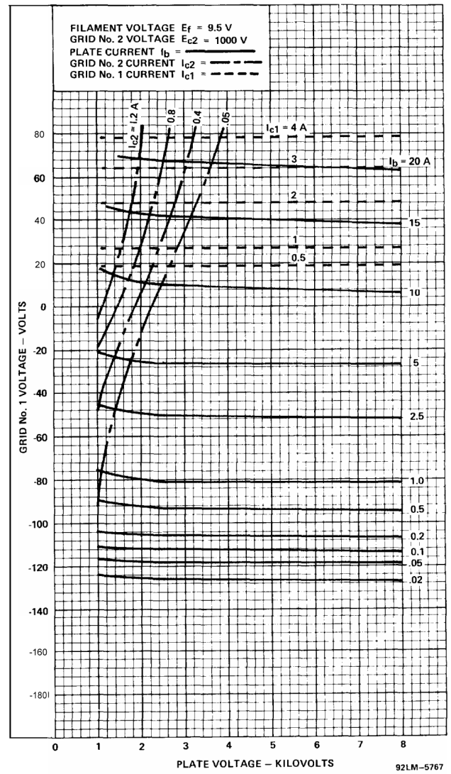
Figure 4 - Typical Constant Current Characteristics
