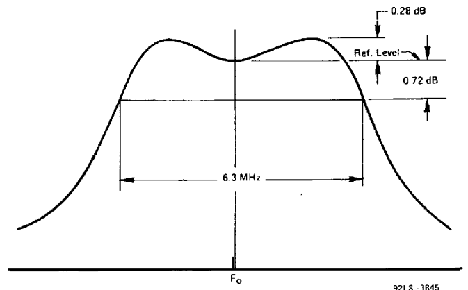
Figure 2 - Bandwidth Characteristics
