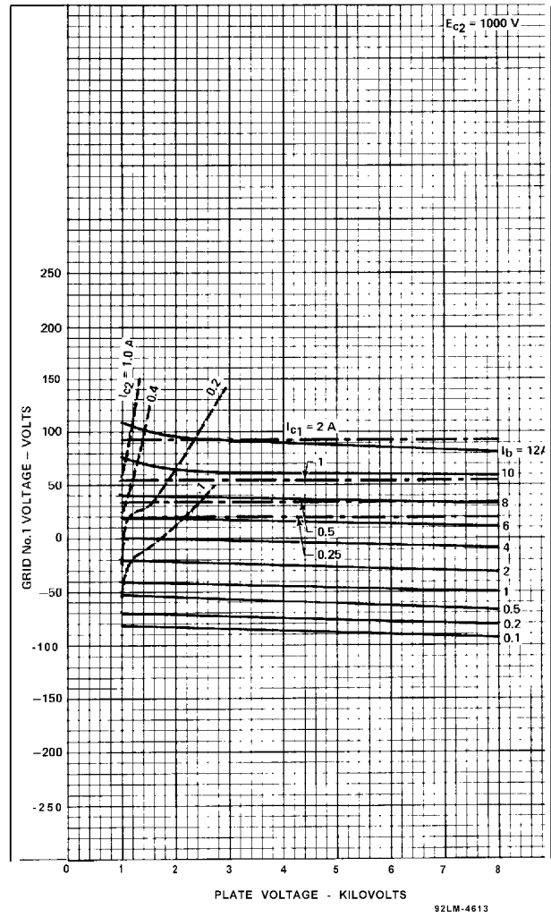
Figure 2 - Typical Constant Current Characteristics E_{c2} = 1000 \text{ V}
