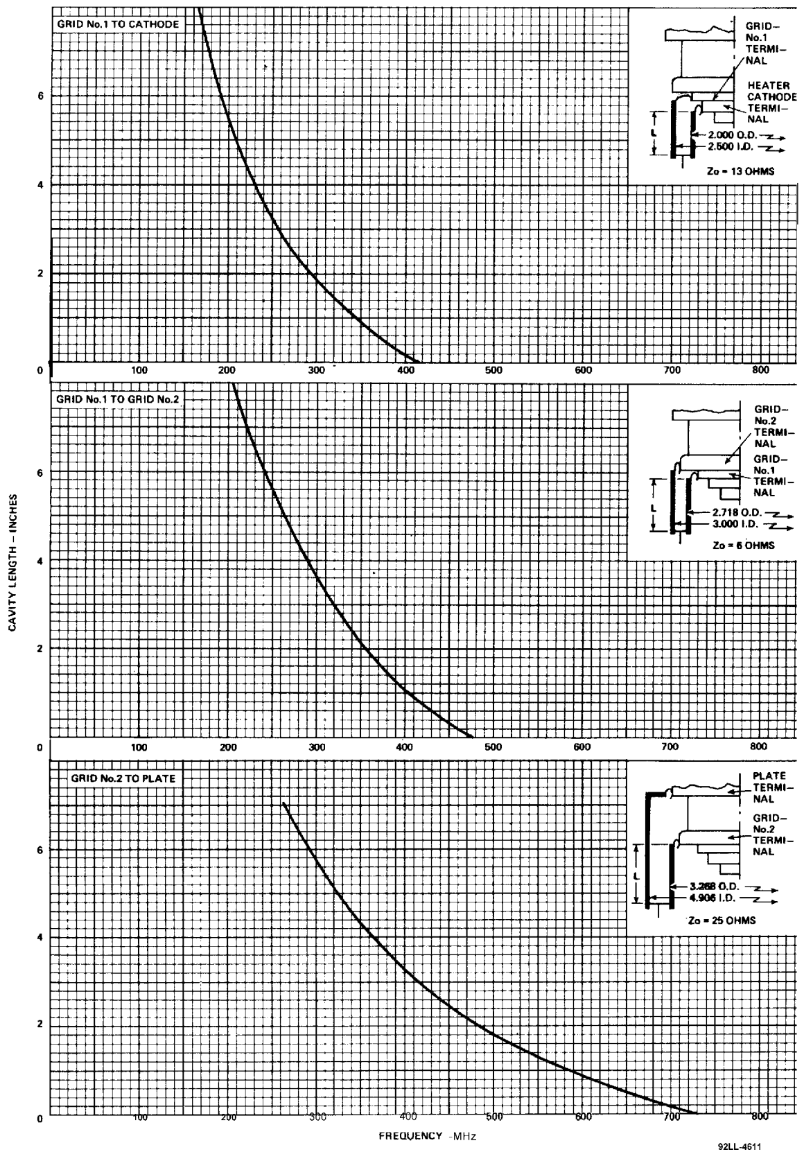
Figure 9 -Tuning Characteristics
