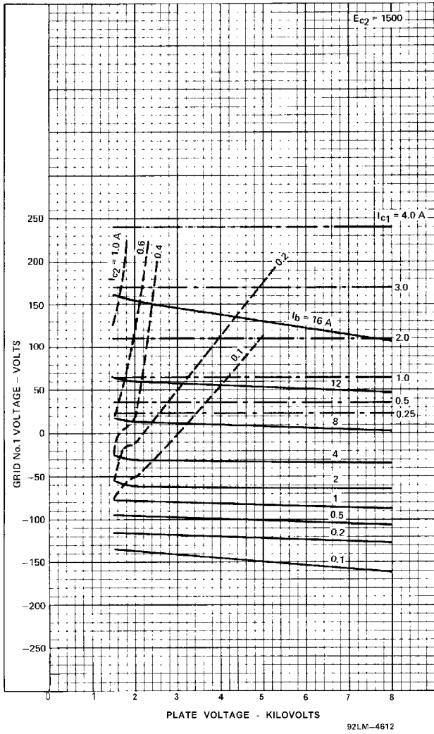
Figure 1 - Typical Constant Current Characteristics E_{c2} = 1500\text{V}
