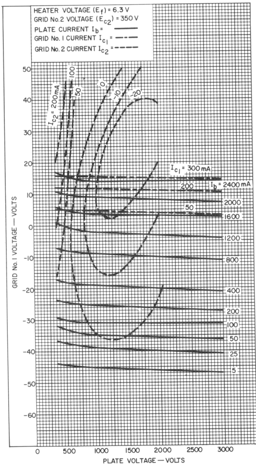
Figure 2 - Typical Constant Current Characteristics ( E_{c2} = 350 \text{ V} )
