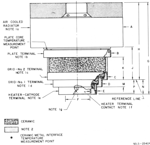
Figure 5 - Dimensional Outline
