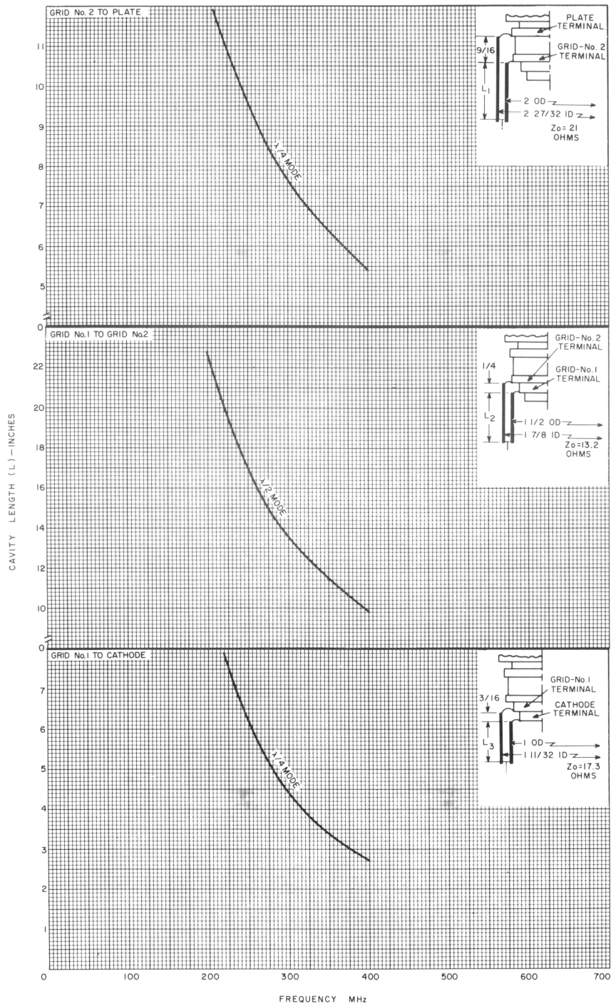
Figure 4 - Electrode Cavity Tuning Characteristics
