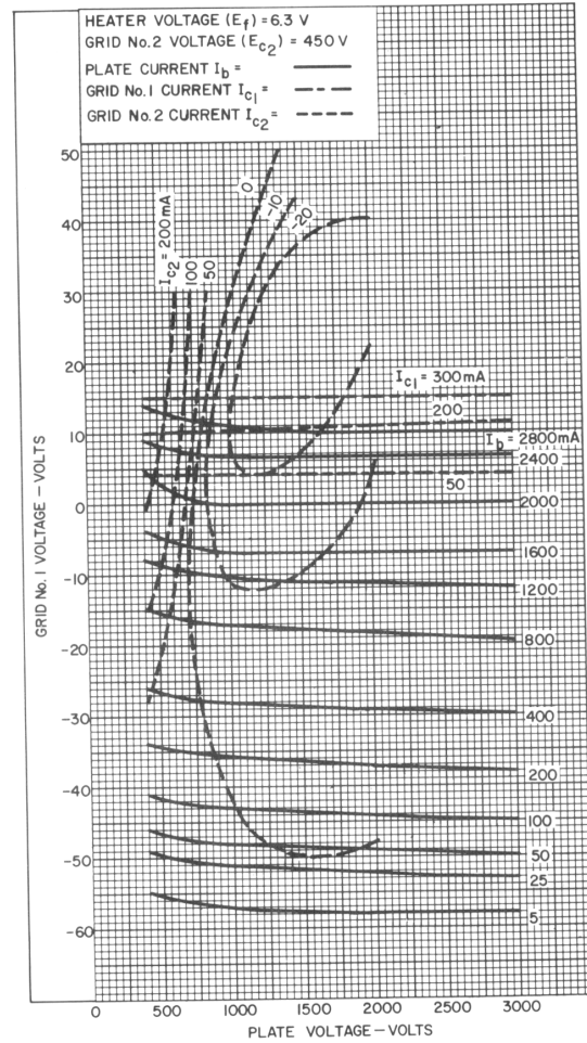
Figure 3 - Typical Constant Current Characteristics ( E_{c2} = 450 \text{ V} )
